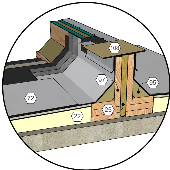
AlphaGuard® BIO Plus Expansion Joint Detail, Structural Concrete Deck Detail 23082
