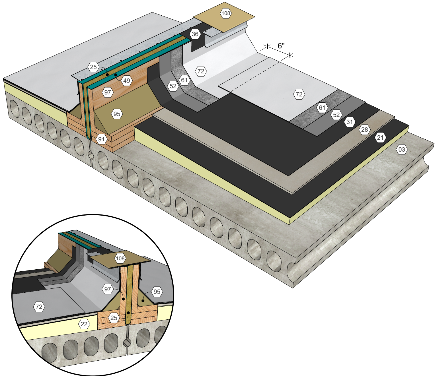
AlphaGuard® BIO Plus Expansion Joint Detail, Precast Concrete Deck Detail 23083
