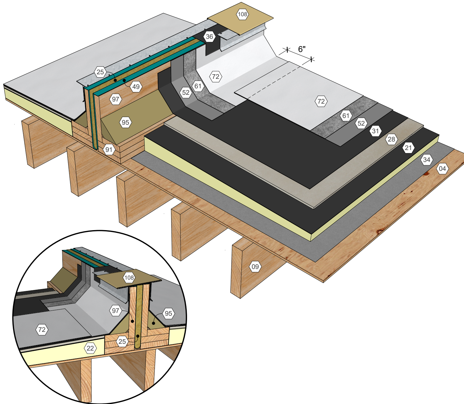
AlphaGuard® BIO Plus Expansion Joint Detail, Wood Deck Detail 23084
