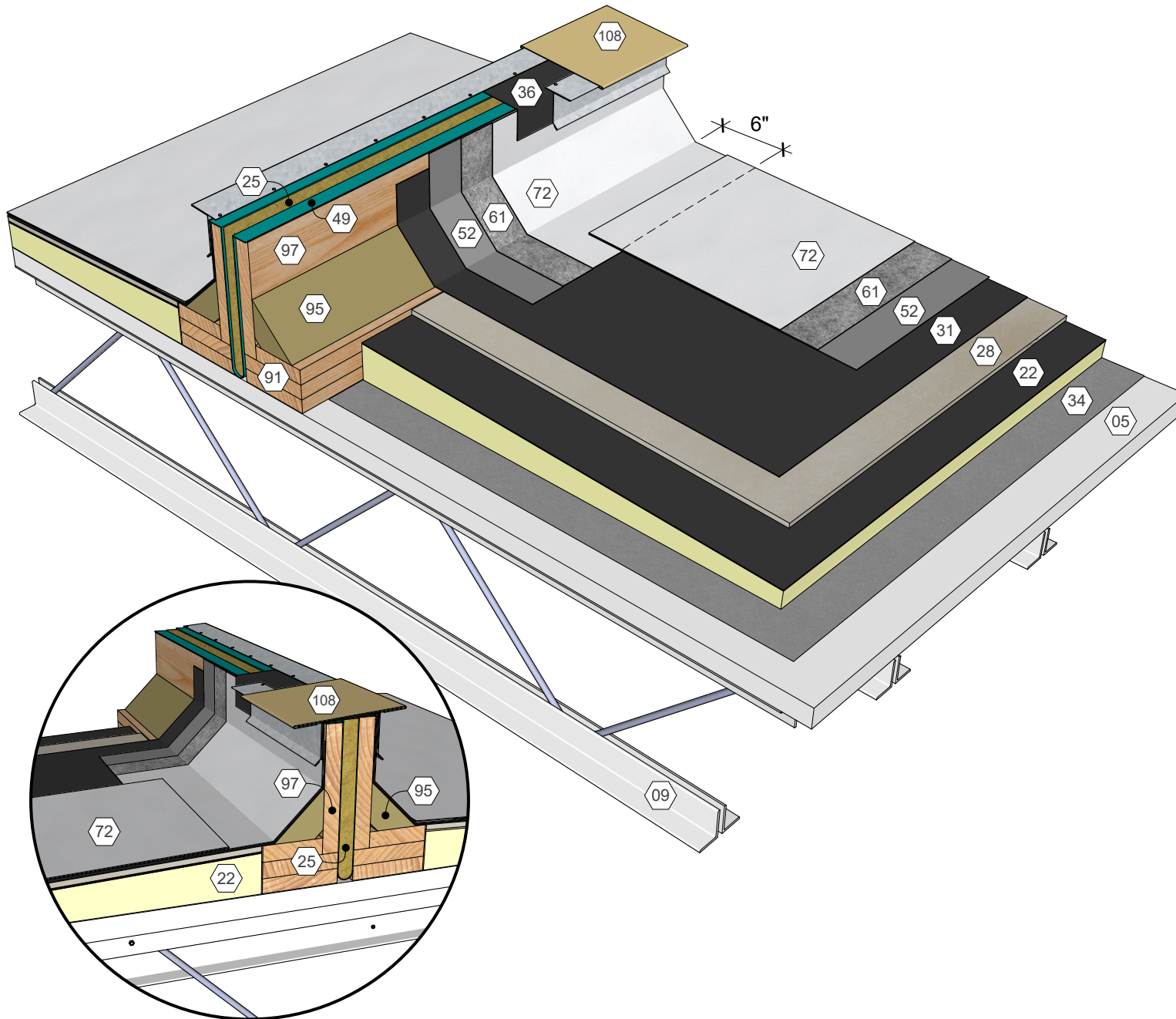
AlphaGuard® BIO Plus Expansion Joint Detail, Gypsum Deck Detail 23085
