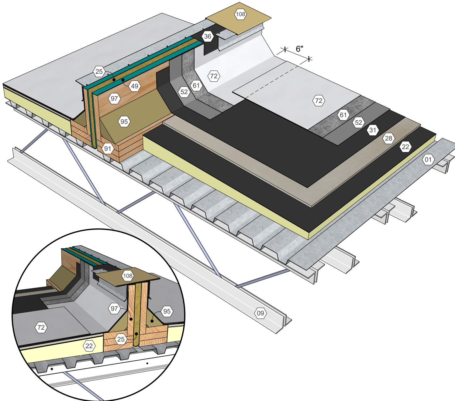
AlphaGuard® BIO Plus Expansion Joint Detail, Metal Deck Detail 23081
